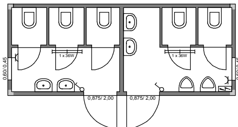
Typ C3S 11 - (LxB) 6,058m x 2,438m; RH = 2,50m
