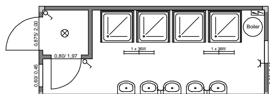
Typ C3S 12 - (LxB) 6,058m x 2,438m; RH = 2,50m
